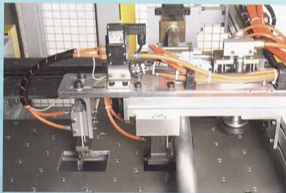
鐵皮檔塊與定位吸盤 Sheet stopper and positioning pad
